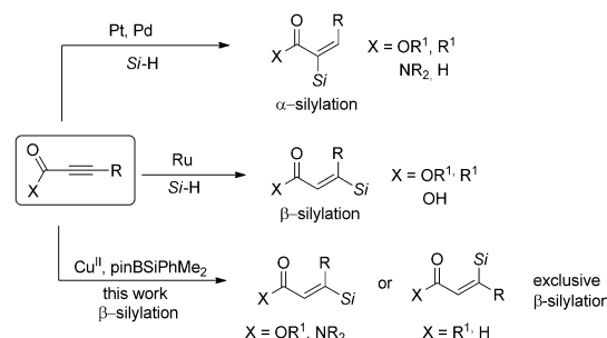
Scheme 1. Strategies toward carbonyl conjugated vinylsilanes.
